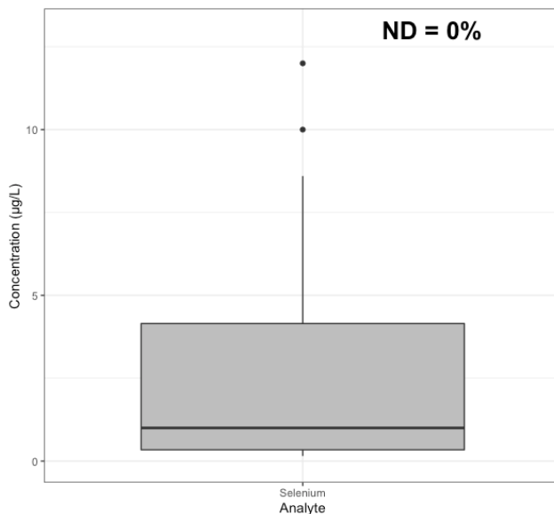
Figure A-3. Box plots generated from 4-county CEDEN data (2010-2021) for total fraction selenium. The Basin Plan WQO for selenium is 5 µg/L; all datapoints above the WQO are associated with Permanente Creek monitoring.
