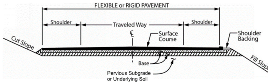
Figure 4-2. Basic Roadway Pavement Layers
