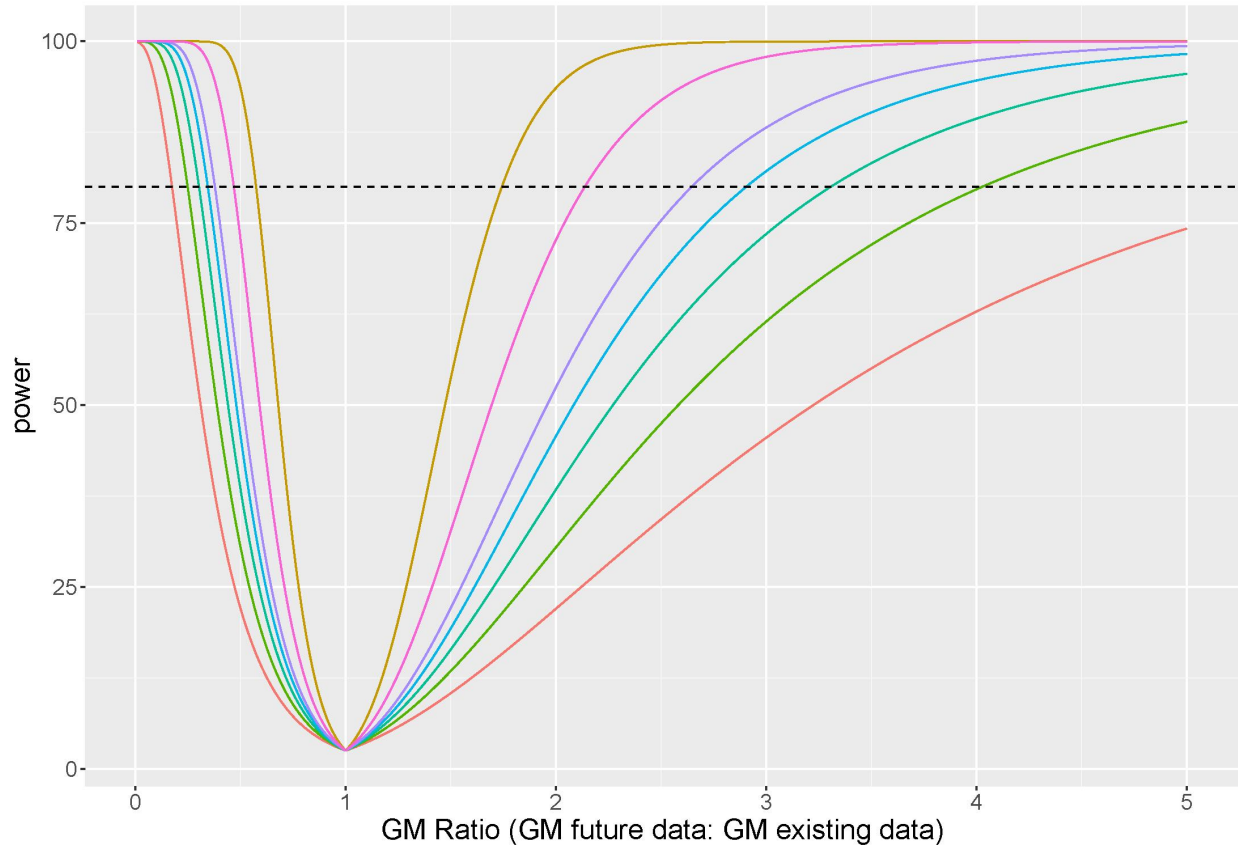
International LID TSS non-parametric power vs. GM_new/GM_orig (n_pre=537) Existing data mean = 22.875; Existing data geomean = 4.936
